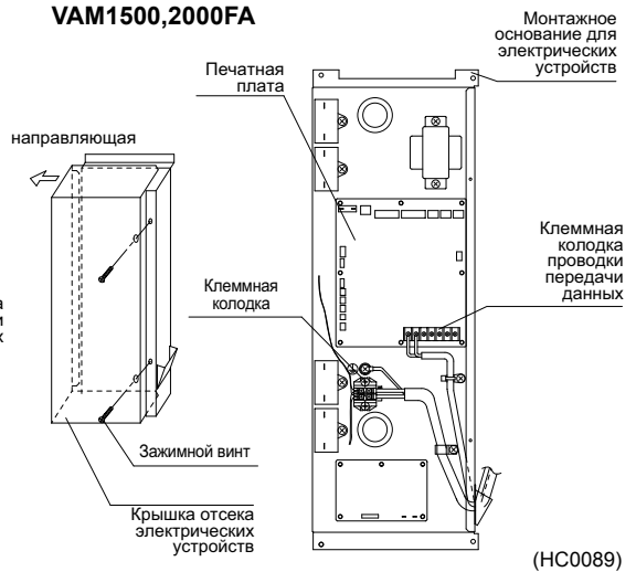
VAM1500,2000FA
